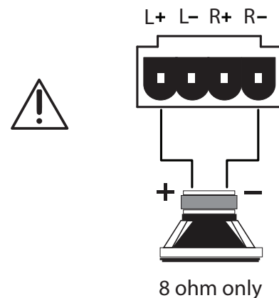
Figure 4 Bridged speaker connection
